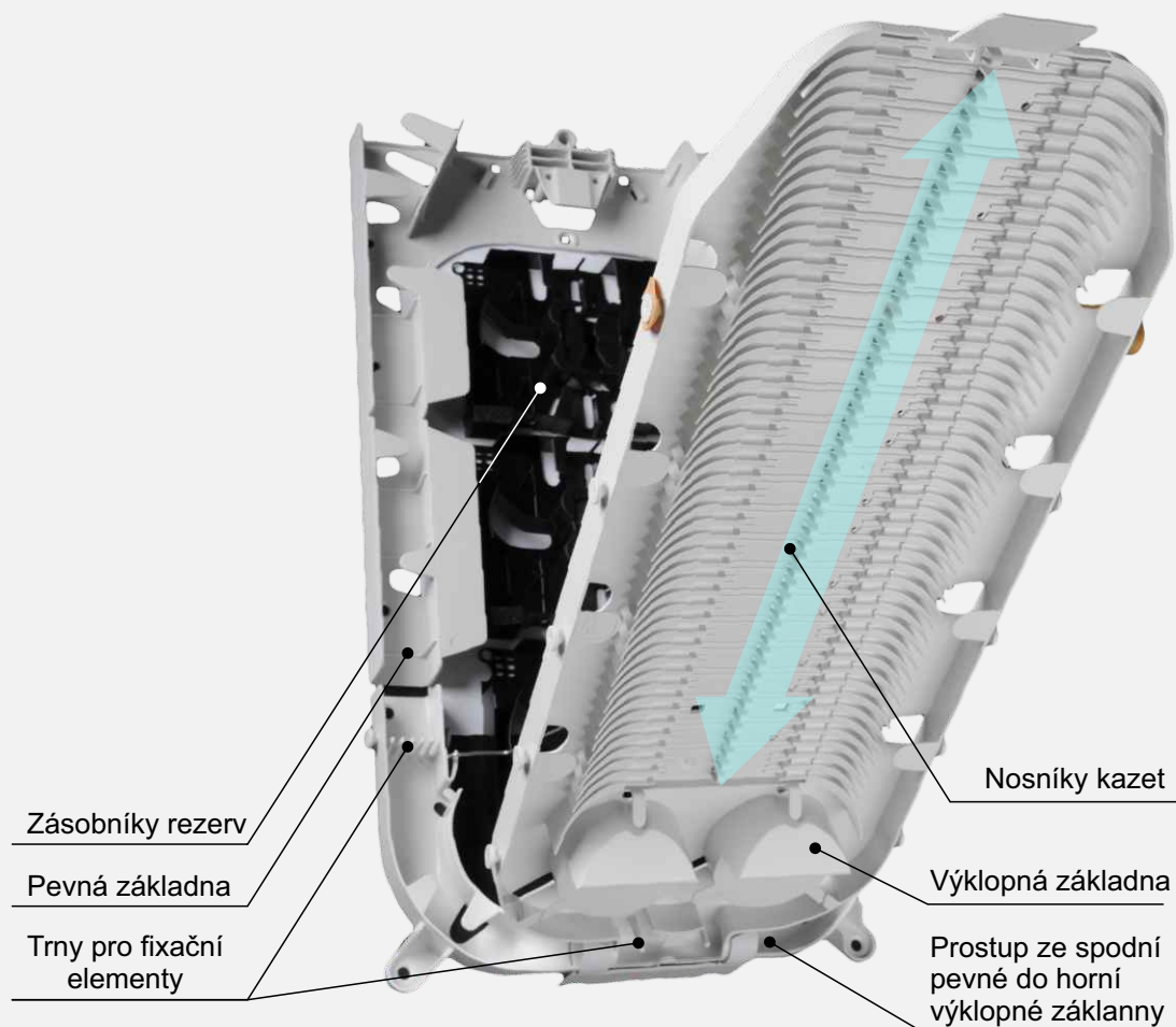
SCM Organizer T3 (48 slotů)
